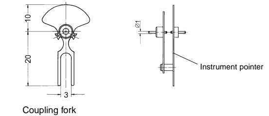
Coupling fork
