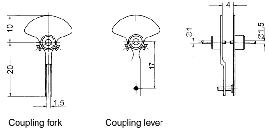
Coupling fork
